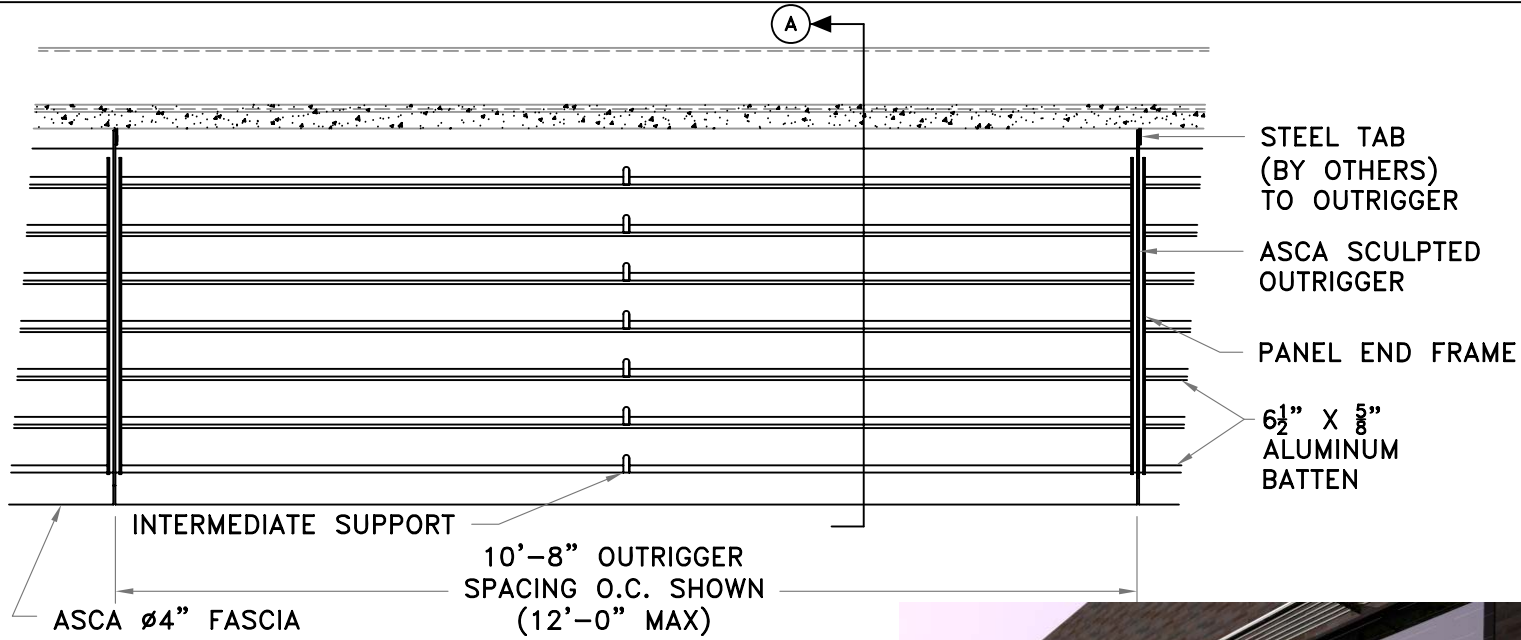
1 PLAN VIEW 1/2" = 1'-0"
