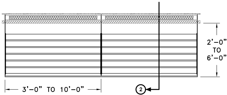
1 PLAN VIEW 1/4" = 1'-0"
