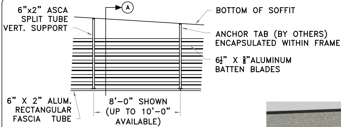
1 ELEVATION VIEW
