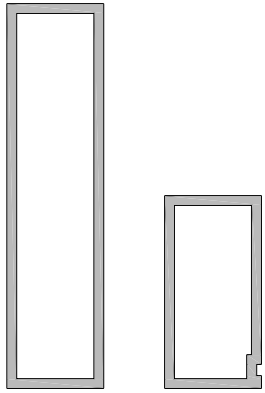
RECTANGULAR TUBES HEIGHTS: 2" TO 8" WIDTHS: 1/2" TO 4" (OPTIONAL ACCENT BAND)
