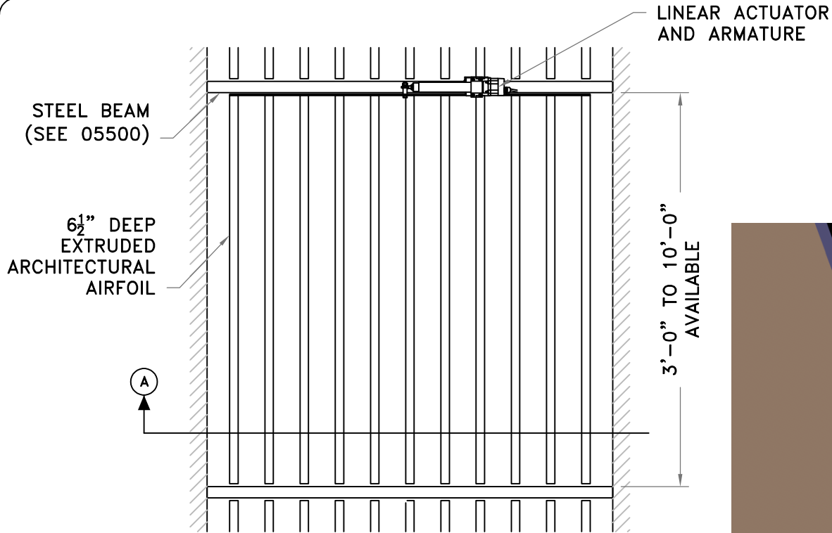
1 PLAN VIEW 1/2" = 1'-0"
