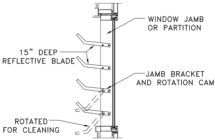
A SECTION VIEW 1/2" = 1'-0"
