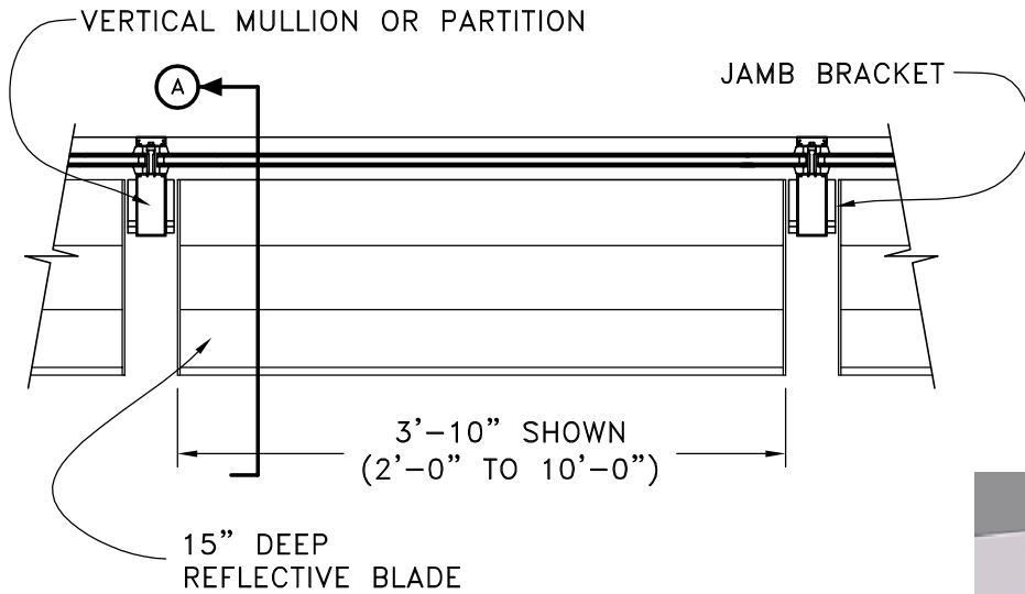
1 PLAN VIEW 3/4" = 1'-0"
