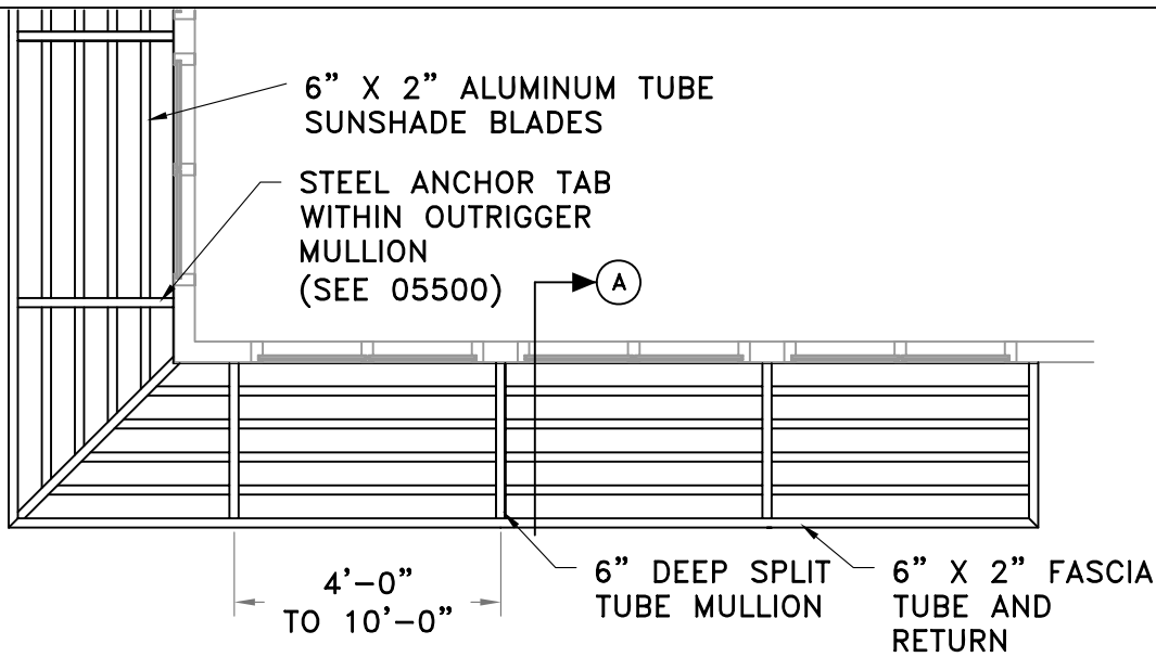
1 PLAN VIEW 1/4" = 1'-0"
