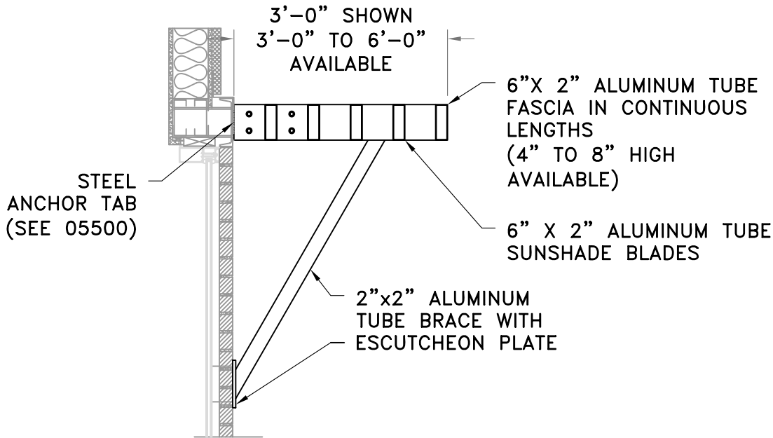
A SECTION VIEW 3/4" = 1'-0"
