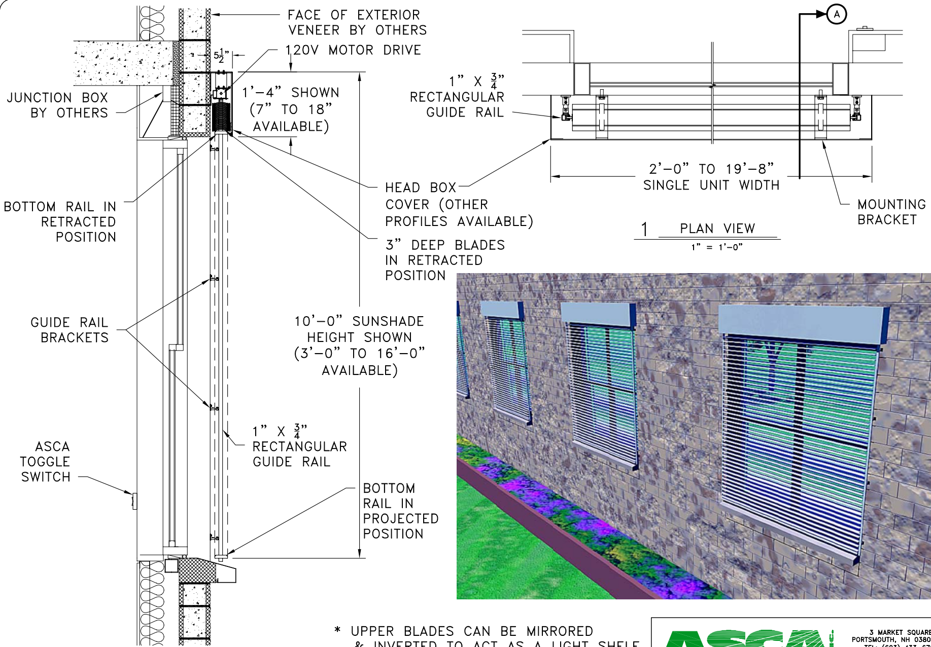
A SECTION VIEW 1/2" = 1'-0"
