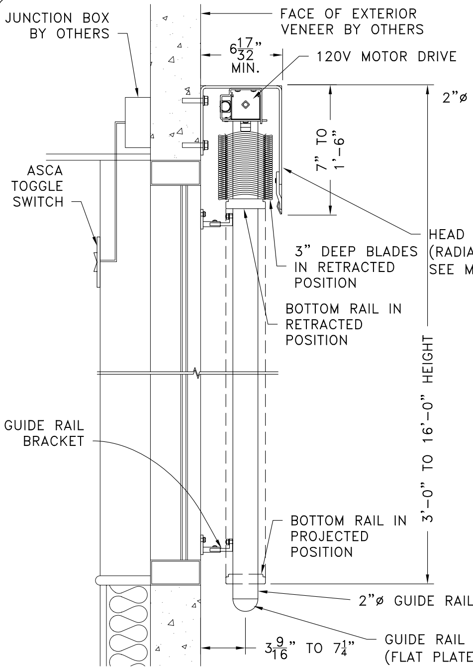
A SECTION VIEW 1 1/2" = 1'-0"
