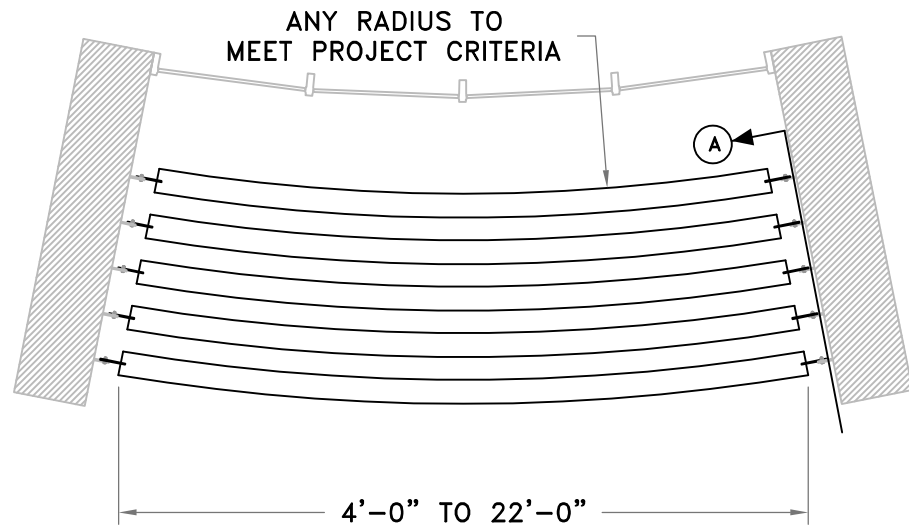
1 PLAN VIEW
